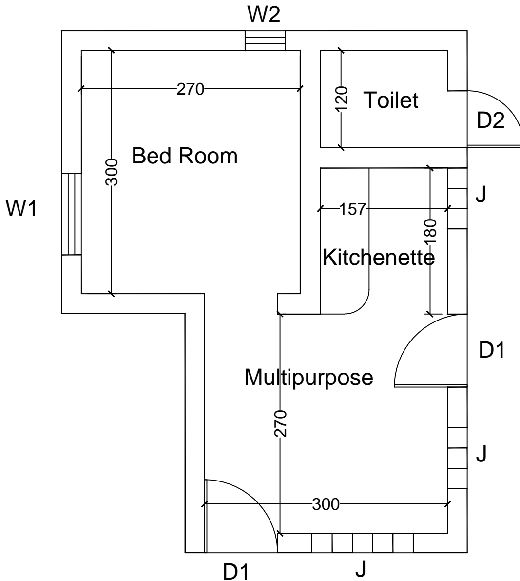
FLOOR PLAN Area: 298 sq.ft
